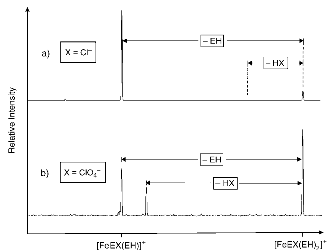
Figure 4. CID spectra of [\text{FeEX}(\text{EH})_2]^+ with \text{X} = {}^{35}\text{Cl} ( E_{\text{CM}} = 1.2 \text{ eV} ) and {}^{35}\text{ClO}_4 ( E_{\text{CM}} = 1.0 \text{ eV} ) and \text{EH} = \mathbf{1a} .
