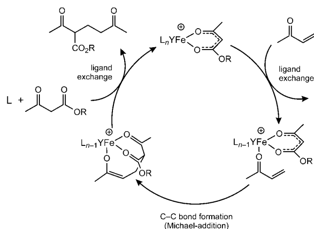
Scheme 1. Proposed mechanistic scheme for the catalytic cycle of the iron(III)-catalyzed Michael addition. Y stands for an additional anionic ligand and L for a neutral ligand. The number n of neutral ligands depends on the hapticity of L to afford an octahedral coordination sphere of the metal center.
