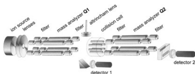
Figure 7. Setup of the VG BIO-Q mass spectrometer.
