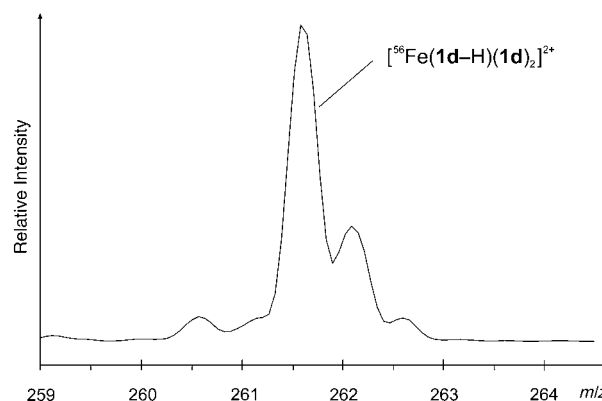
Figure 1. Dicationic [\text{FeE}(\text{EH})_2]^{2+} observed in the cation ESI spectrum of a dilute solution of \text{Fe}(\text{ClO}_4)_3 and 1d in \text{CH}_2\text{Cl}_2 .
