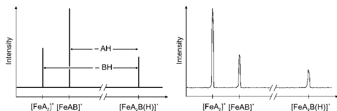
Figure 6. Comparison of a hypothetical 1:2 fragmentation pattern expected for the collision induced dissociation of an [\text{FeA}_2\text{B}(\text{H})]^+ complex with equally bound esters AH and BH (left) with the actual fragmentation pattern observed in the case of AH= 1b and BH= 1c at a collision energy of E_{\text{CM}} = 3.3 eV (right).
