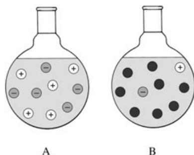
Figure 2. Schematic representation of the possible situation in solution after dissolving an FeX 3 salt and ≥3 equivalents of ester in dichloromethane. A: solution with predominantly charged complexes. B: solution with predominantly neutral complexes and only small amounts of ions. ⊖ represents any negatively charged particles in solution, ⊕ any positively charged particles and ● any neutral complexes.
